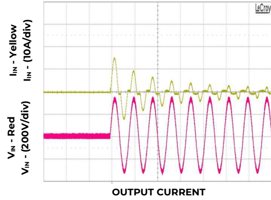
Figure 2. Inrush current V_{IN} = 230V_{AC} , 0°C phase angle
